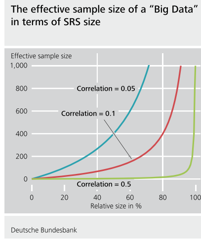
FIG. 2. Effective sample size n_{\text{eff}}^* as a function of the relative size (sampling rate) f . [I thank Dr. Jens Mehrhoff for his permission to use this figure from Mehrhoff (2016).]
