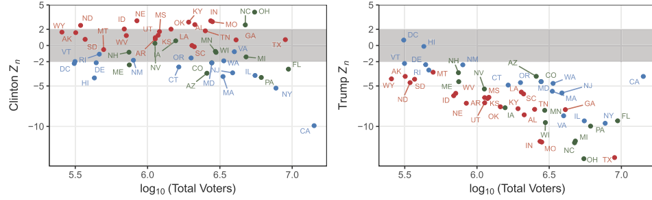
FIG. 7. Estimates of Z_n = \frac{\hat{p} - p}{\sqrt{\hat{p}(1-\hat{p})/n}} : The conventional 95% confidence interval region |Z_n| \leq 2 is indicated in gray.
