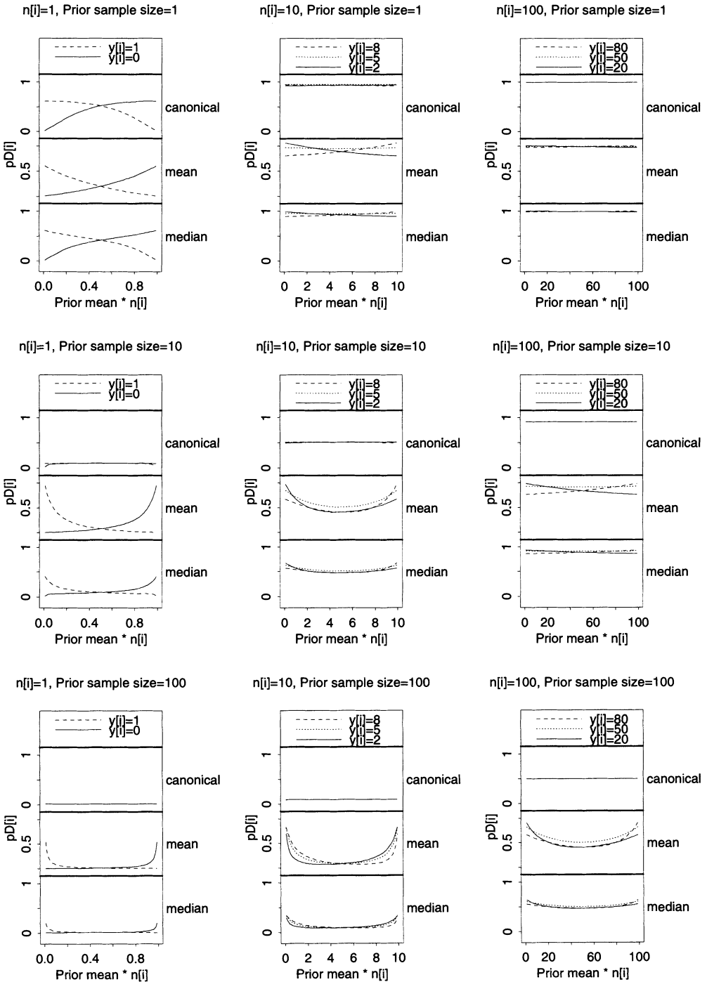
Fig. 1. Binomial likelihood—contribution of the i th group to the effective number of parameters under various parameterizations (canonical p_{D_i}^{\theta} , mean p_{D_i}^{\mu} and median p_{D_i}^{\text{med}} ) as a function of the data (sample size n_i and observed proportion y_i/n_i ) and prior (effective prior sample size a + b and prior mean a/(a + b) ): we are seeking agreement between alternative parameterizations with little dependence on data
