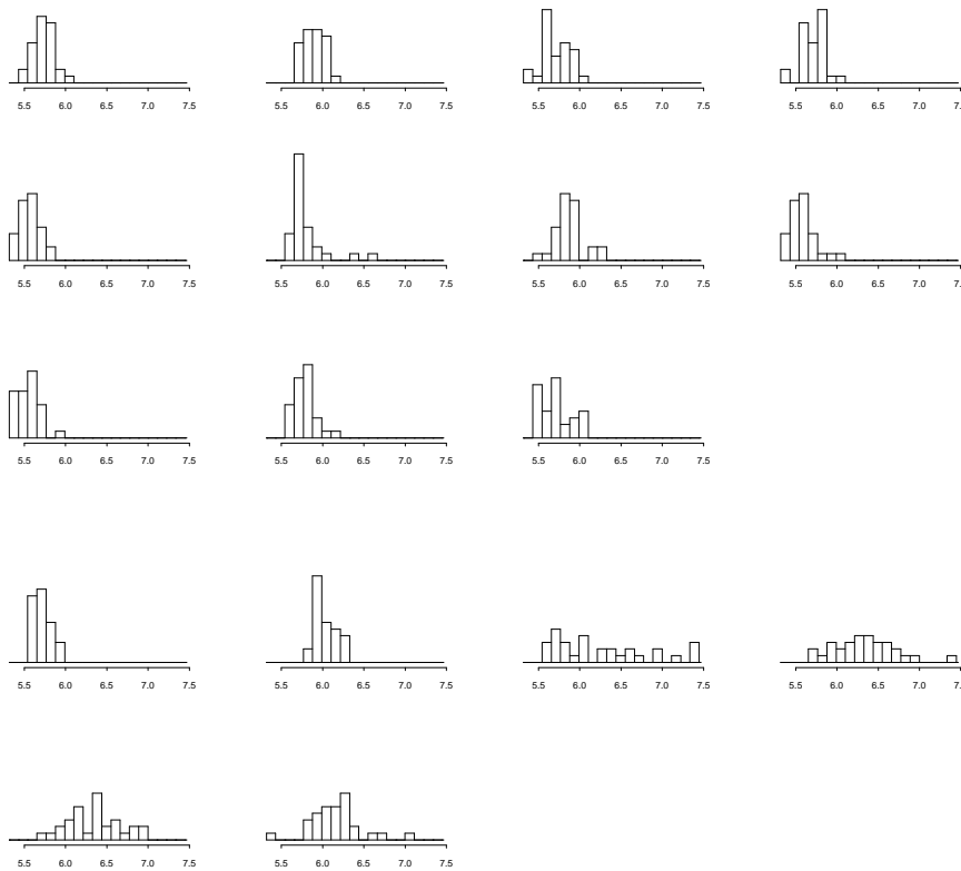
Figure 0.1. (a) Log response times for 11 non-schizophrenic individuals, (b) Log response times for 6 schizophrenic individuals. All histograms are on a common scale.
