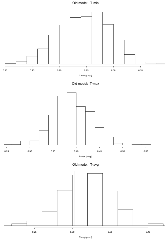
Figure 0.2. Posterior predictive distributions and observed values for three test statistics: the smallest, average, and largest observed within-schizophrenic variances. The vertical line on each histogram represents the observed value of the test statistic.
