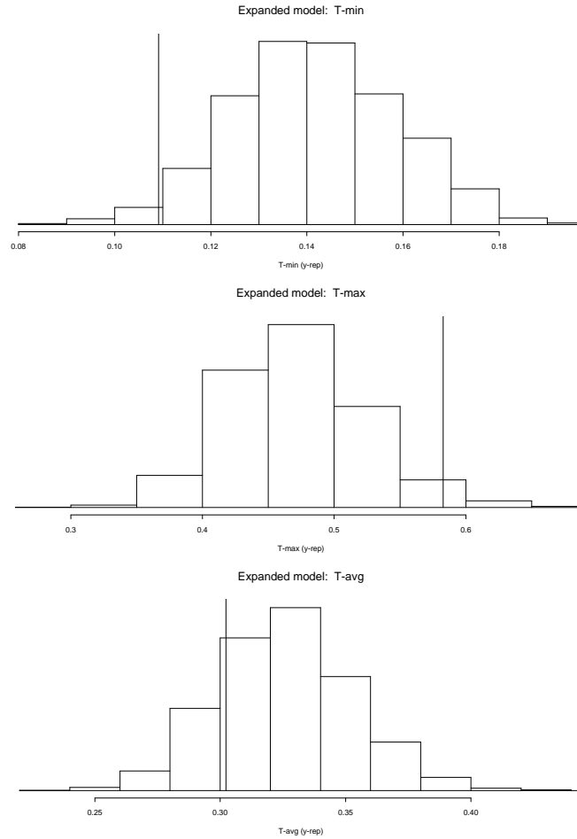
Figure 0.3. Posterior predictive distributions, under the expanded model, for three test statistics: the smallest, average, and largest observed within-schizophrenic variances. The vertical line on each histogram represents the observed value of the test statistic.
