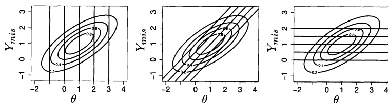
Figure 1. Sampling directions (solid lines) for ASIS in the toy model with Y_{obs} = 1 and V = 1 . Left: Step 1, conditional draw along the lines \theta = \text{const} . Center: Step 2, conditional draw along Y_{mis} - \theta = \text{const} . Right: Step 2, conditional draw along Y_{mis} = \text{const} . The ellipses are contours of the posterior distribution p(\theta, Y_{mis}|Y_{obs}) .
