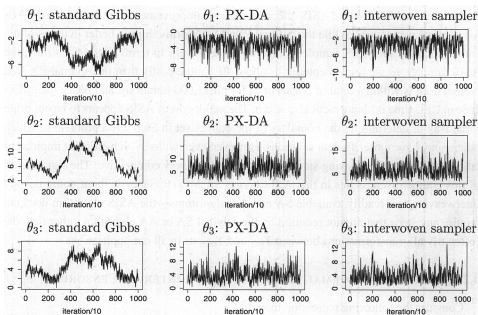
Figure 8. Comparing standard Gibbs with the optimal PX-DA and the interwoven sampler for the lupus nephritis data: trajectories of the draws.
