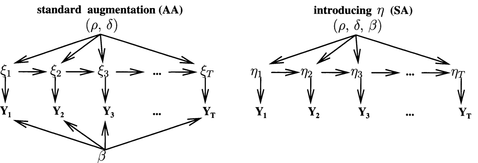
Figure 3. Change in dependence structure among the variables after introducing \eta . Left: structure of the original model, where \xi are the missing data and are an AA for \beta . Right: structure of the transformed model (3.4)–(3.5), where \eta are the missing data and are an SA for \beta . The arrows indicate how data could have been generated by sampling from the relevant conditional distributions (e.g., Y is generated conditional on \xi_1, \dots, \xi_T and \beta in the standard augmentation).
