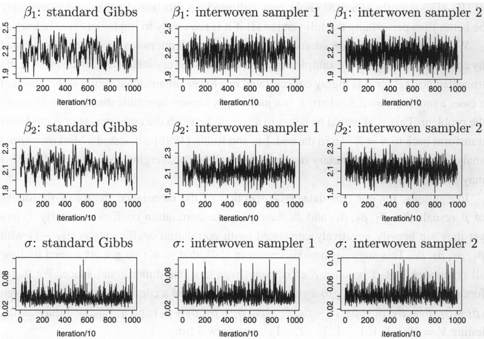
Figure 11. Comparing standard Gibbs with two versions of interweaving for simulated data: trajectories of the draws.
